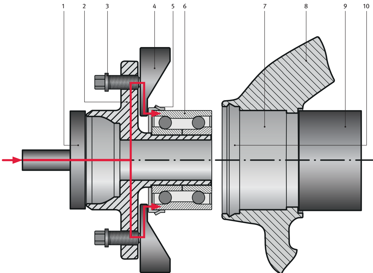
Path of forces during pressing-in process with mounted clamps
